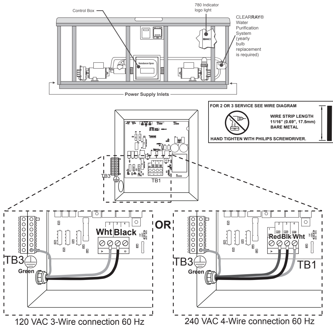
Figure 12 The Spa Equipment Compartment (spa features subject to change without notice. Component locations vary by model. 780 Dover model shown.)
