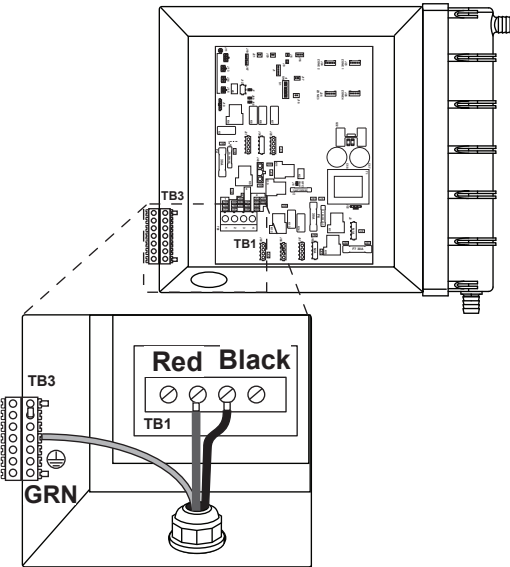
Figure 5 3-wire/240 VAC connection ( Hard Wired Connections Only )
