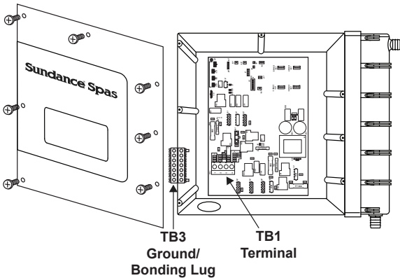
Figure 4: The Control Box for 3-wire, 240 VAC connection (The location of the TB1 terminal may vary between models.)
